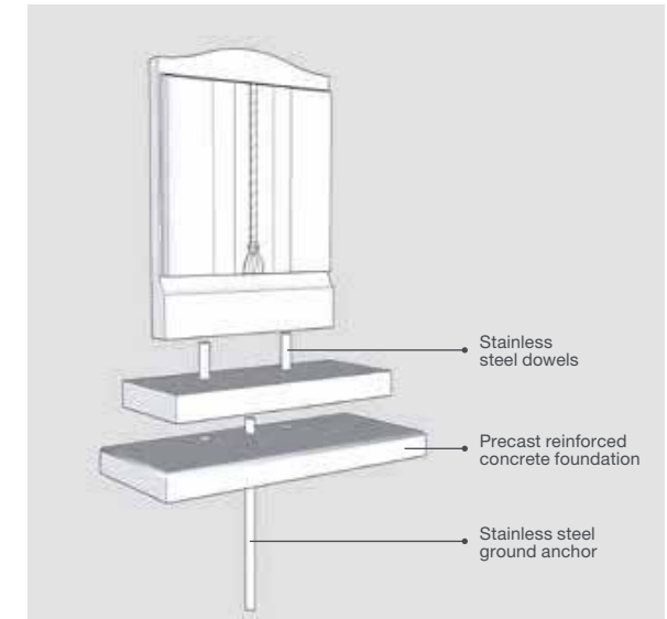
Ground Anchor Fixing Method
